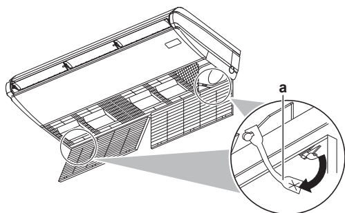
a Strop
